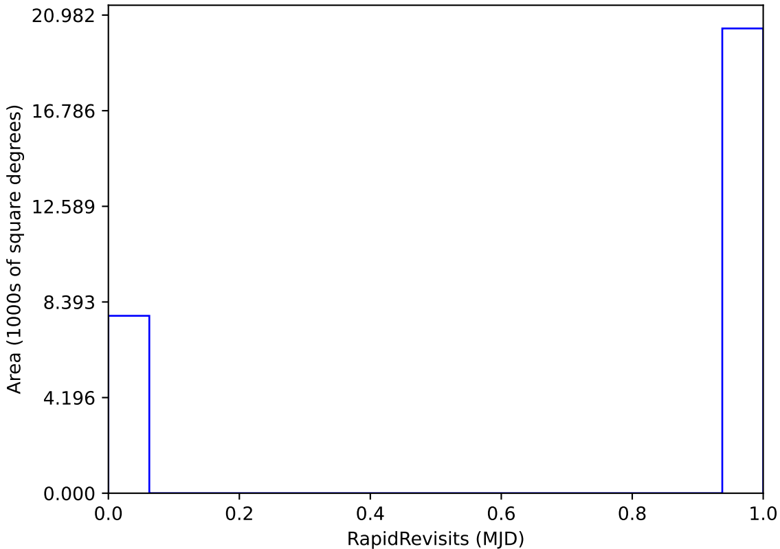
too_elab_r32_d3_giz_v3.4_10yrs : RapidRevisits
