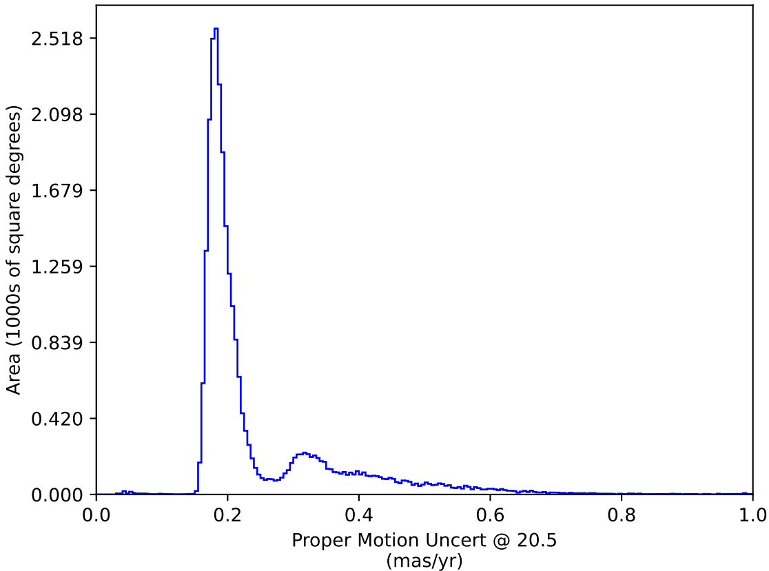
too_elab_r32_d3_giz_v3.4_10yrs : Proper Motion Uncert @ 20.5
