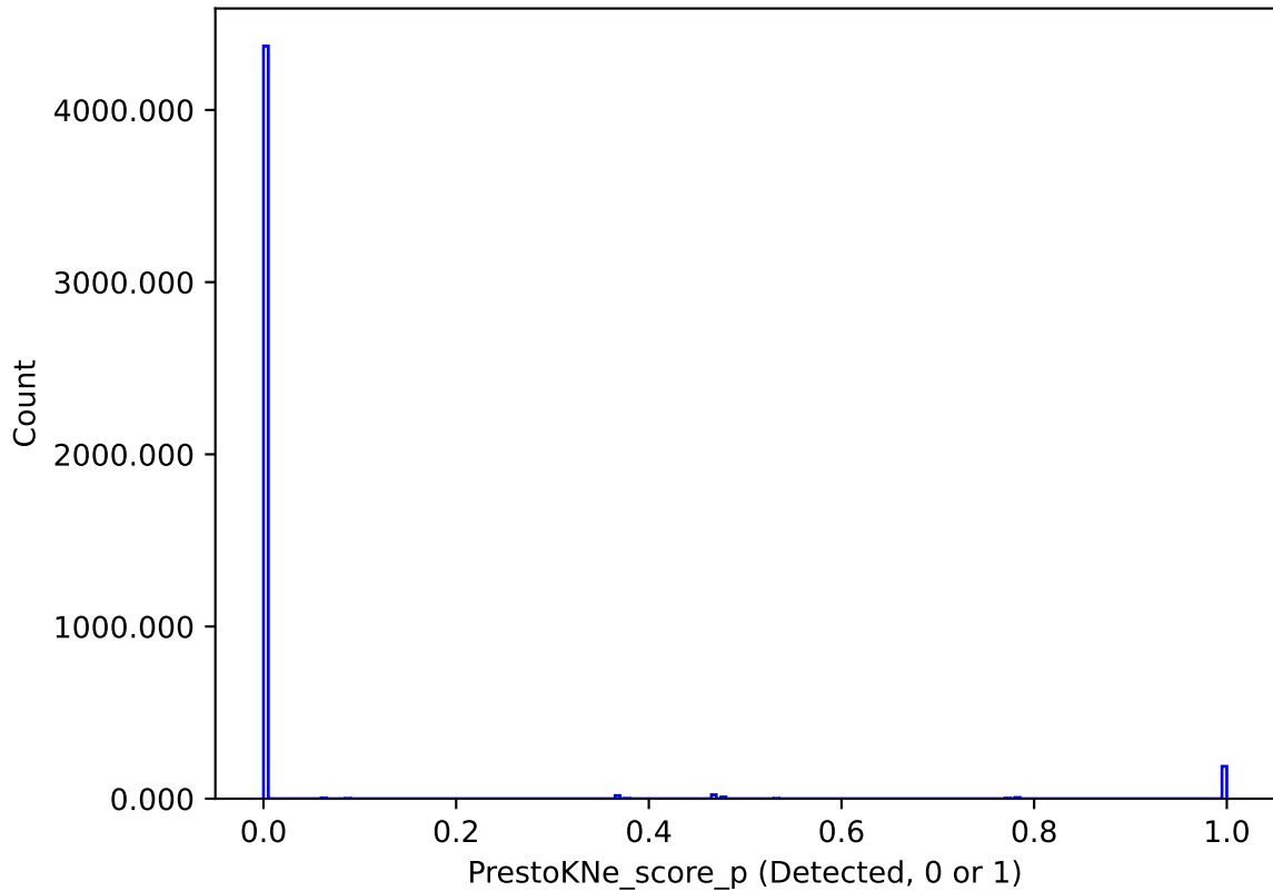
too_elab_r32_d3_giz_v3.4_10yrs : PrestoKNe_score_p
