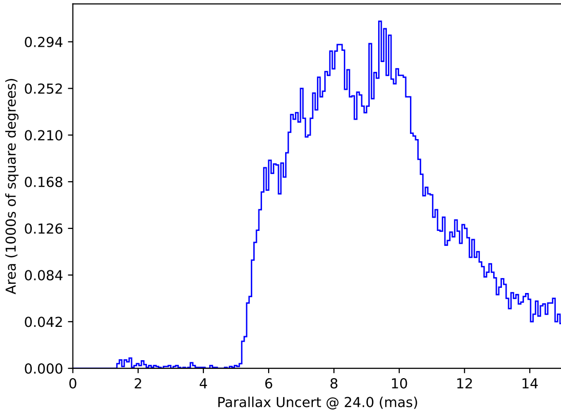
too_elab_r32_d3_giz_v3.4_10yrs : Parallax Uncert @ 24.0
