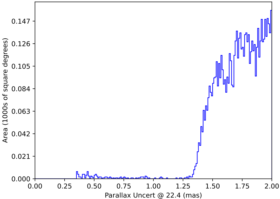
too_elab_r32_d3_giz_v3.4_10yrs : Parallax Uncert @ 22.4
