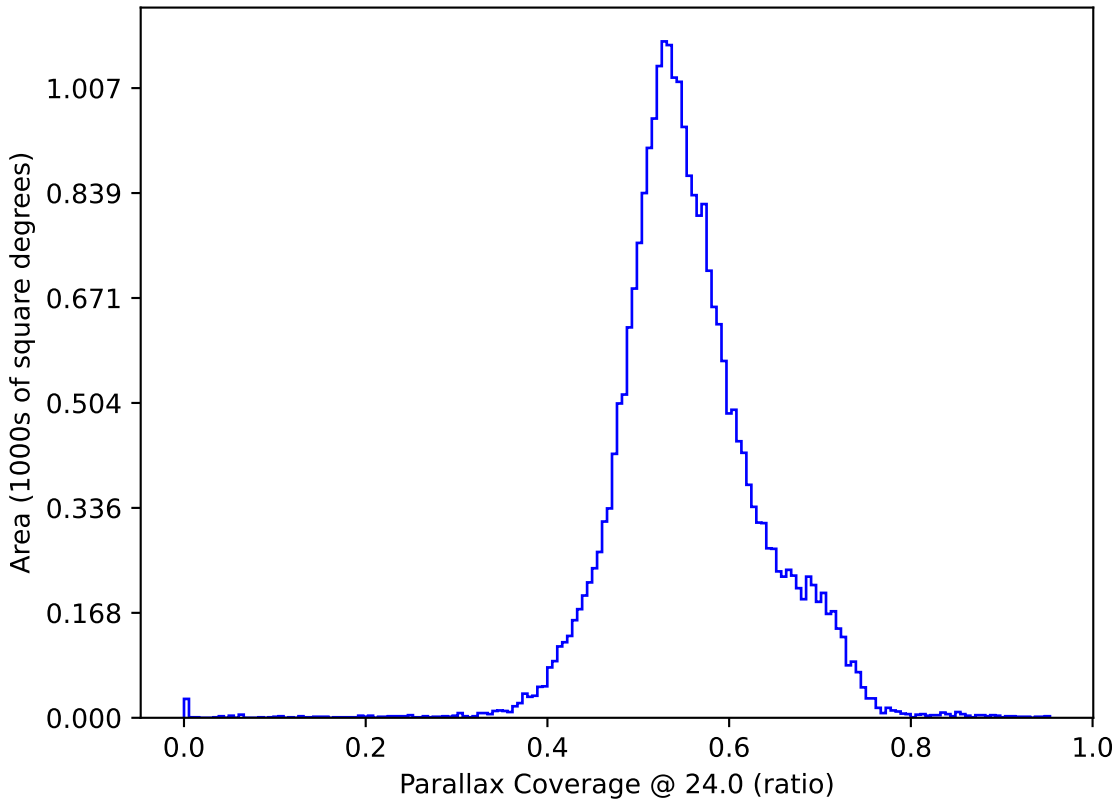
too_elab_r32_d3_giz_v3.4_10yrs : Parallax Coverage @ 24.0
