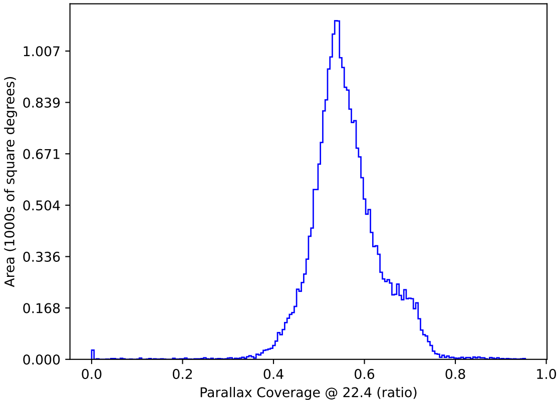
too_elab_r32_d3_giz_v3.4_10yrs : Parallax Coverage @ 22.4
