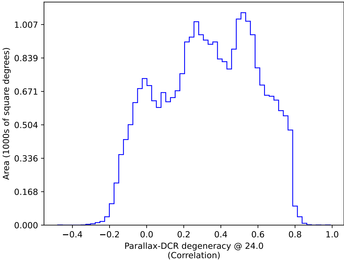
too_elab_r32_d3_giz_v3.4_10yrs : Parallax-DCR degeneracy @ 24.0
