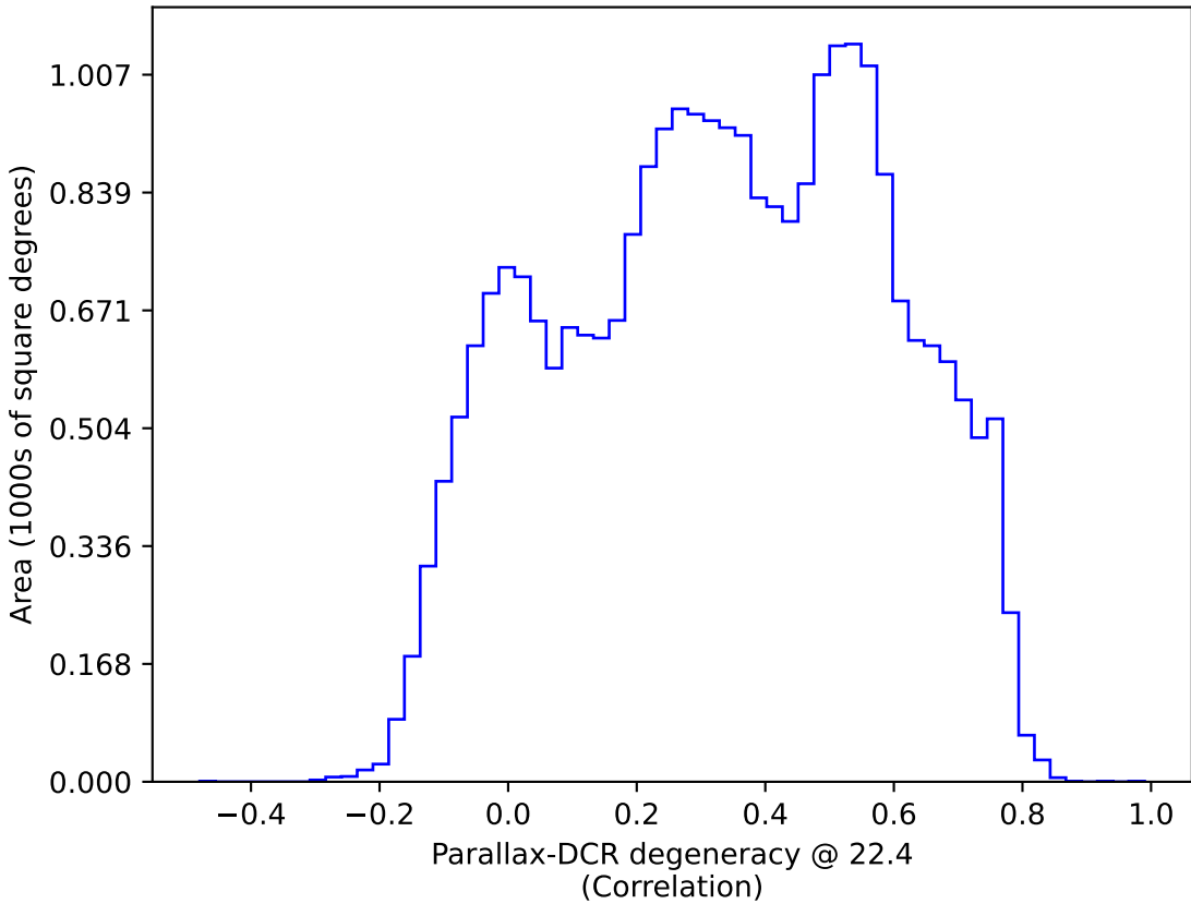
too_elab_r32_d3_giz_v3.4_10yrs : Parallax-DCR degeneracy @ 22.4
