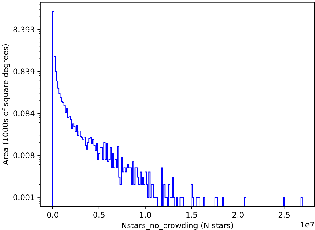
too_elab_r32_d3_giz_v3.4_10yrs i: Nstars_no_crowding
