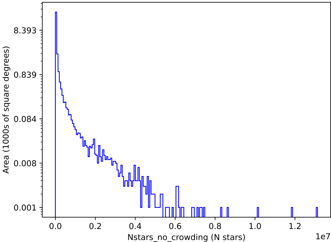
too_elab_r32_d3_giz_v3.4_10yrs g: Nstars_no_crowding
