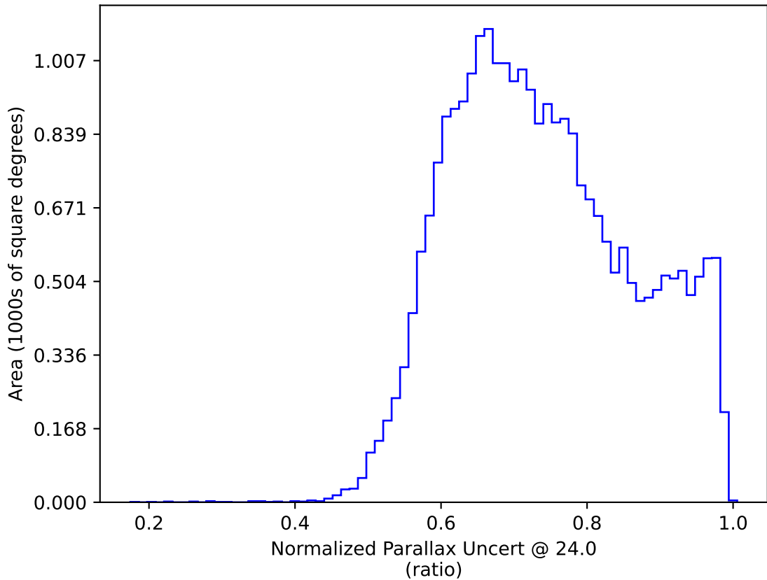
too_elab_r32_d3_giz_v3.4_10yrs : Normalized Parallax Uncert @ 24.0
