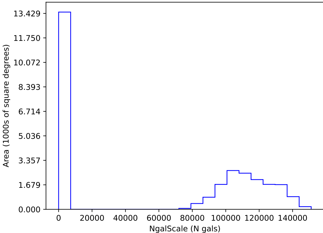
too_elab_r32_d3_giz_v3.4_10yrs i: NgalScale
