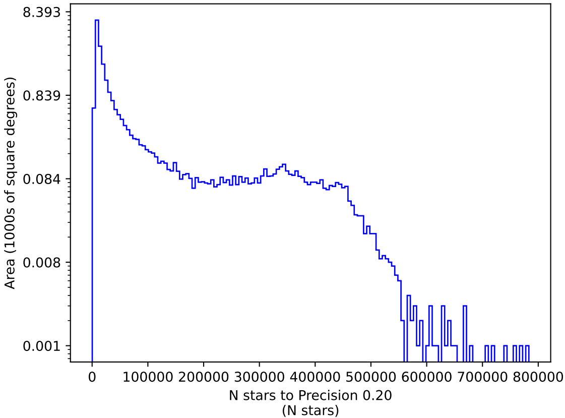
too_elab_r32_d3_giz_v3.4_10yrs y: N stars to Precision 0.20
