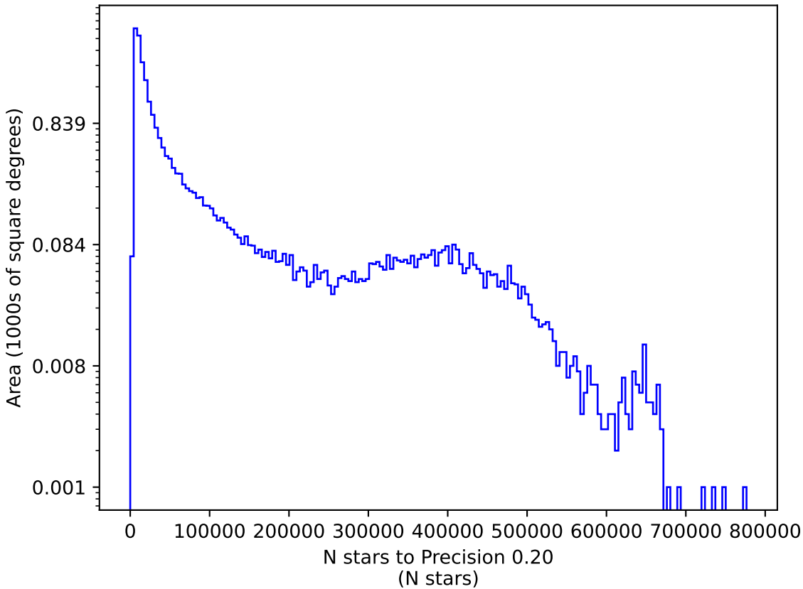
too_elab_r32_d3_giz_v3.4_10yrs r: N stars to Precision 0.20
