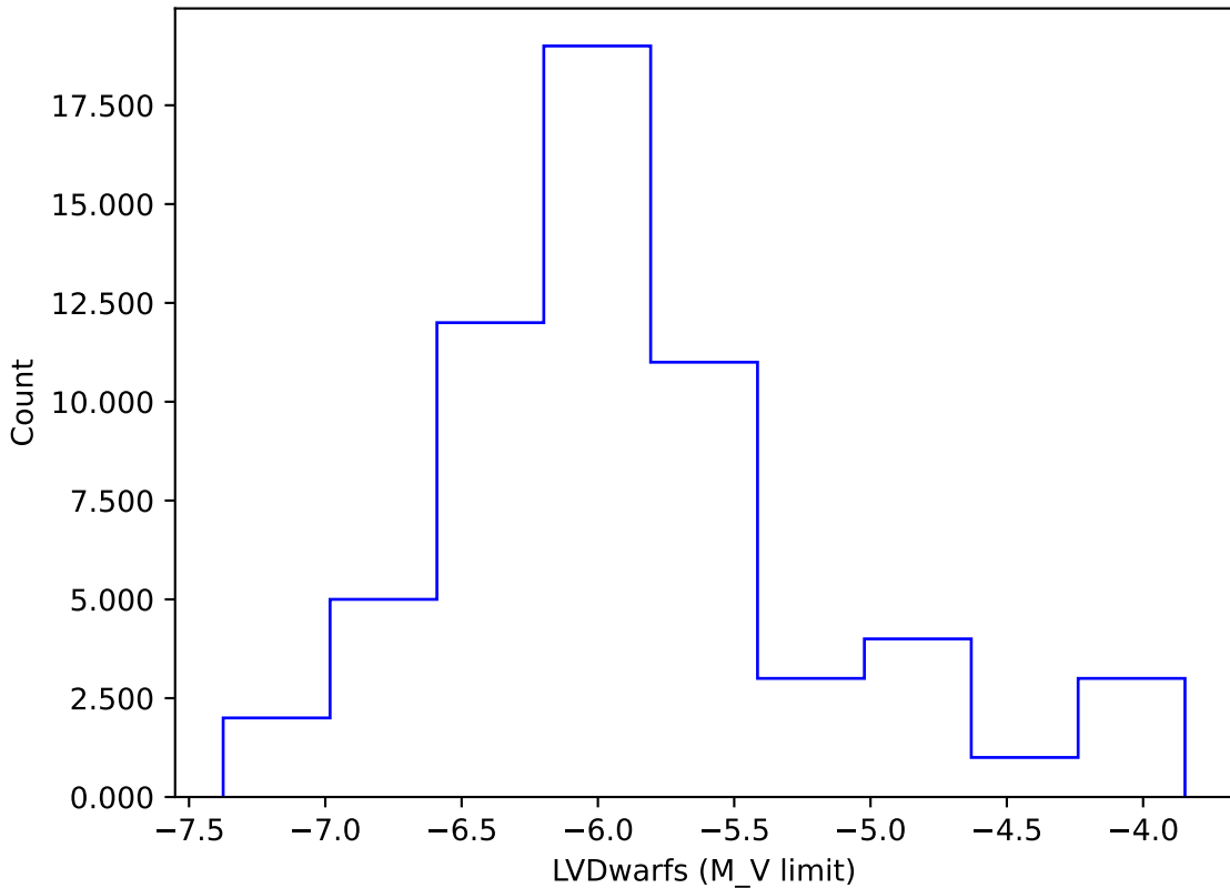
too_elab_r32_d3_giz_v3.4_10yrs gi: LVDwarfs
