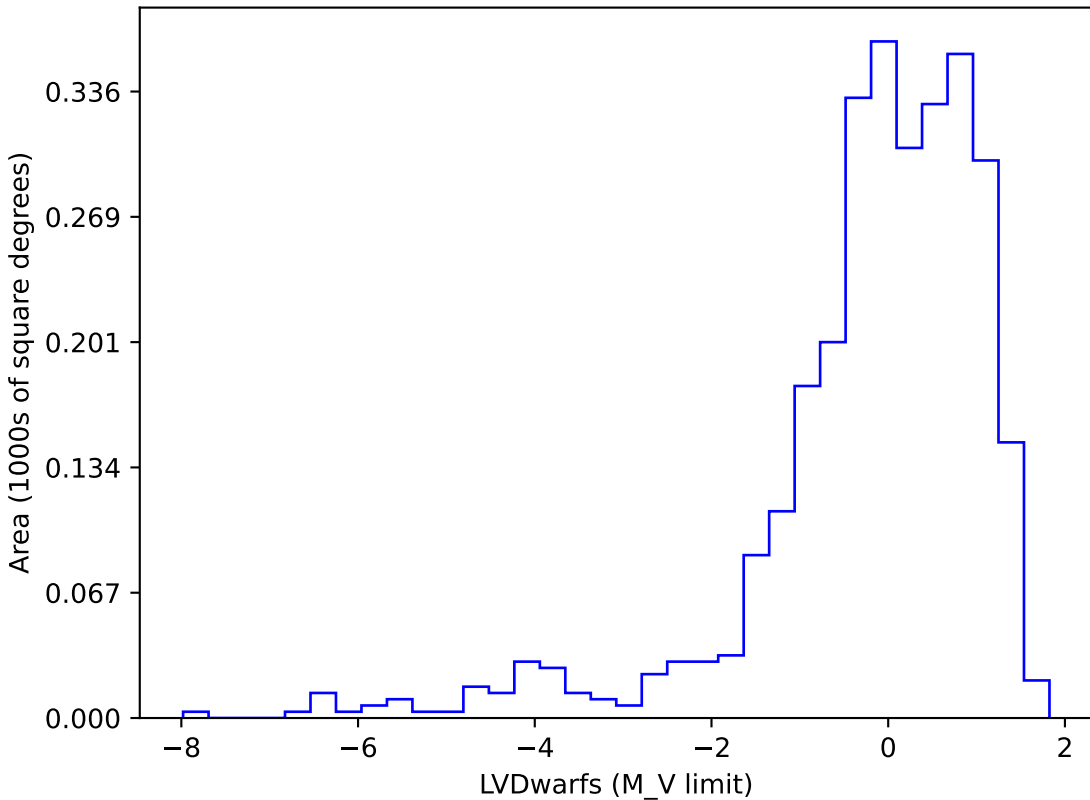
too_elab_r32_d3_giz_v3.4_10yrs gi SCP: LVDwarfs
