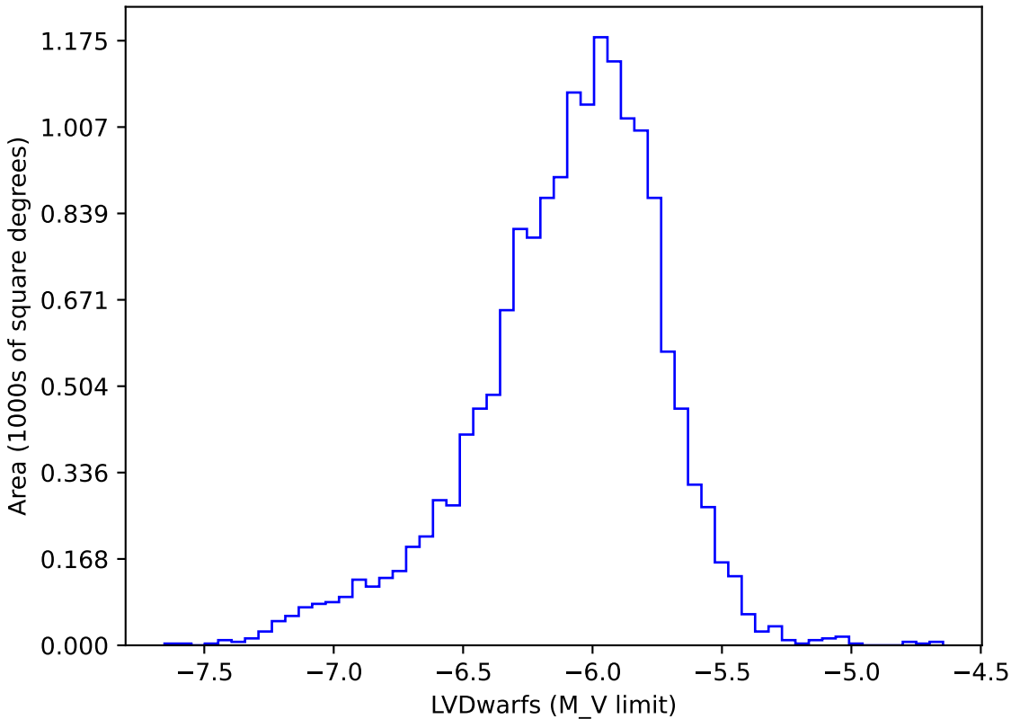
too_elab_r32_d3_giz_v3.4_10yrs gi: LVDwarfs
