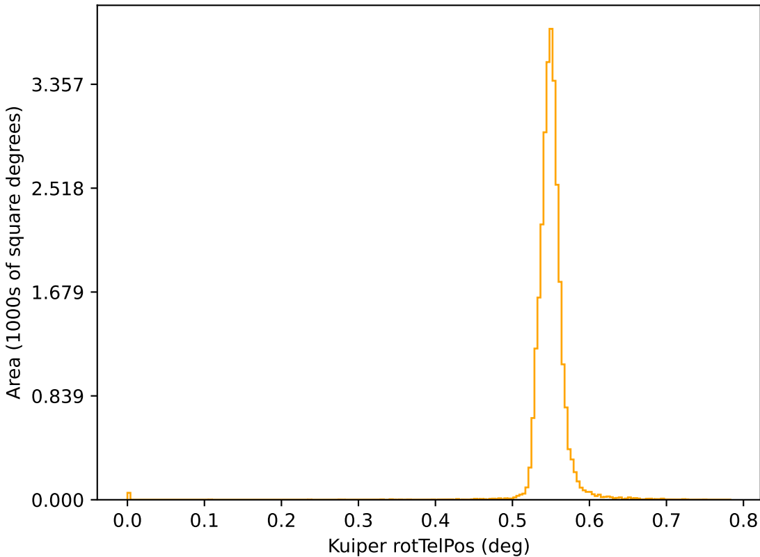
too_elab_r32_d3_giz_v3.4_10yrs r: Kuiper rotTelPos
