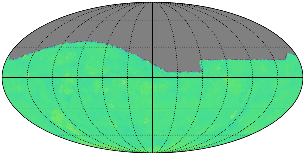
too_elab_r32_d3_giz_v3.4_10yrs g: Kuiper rotTelPos
