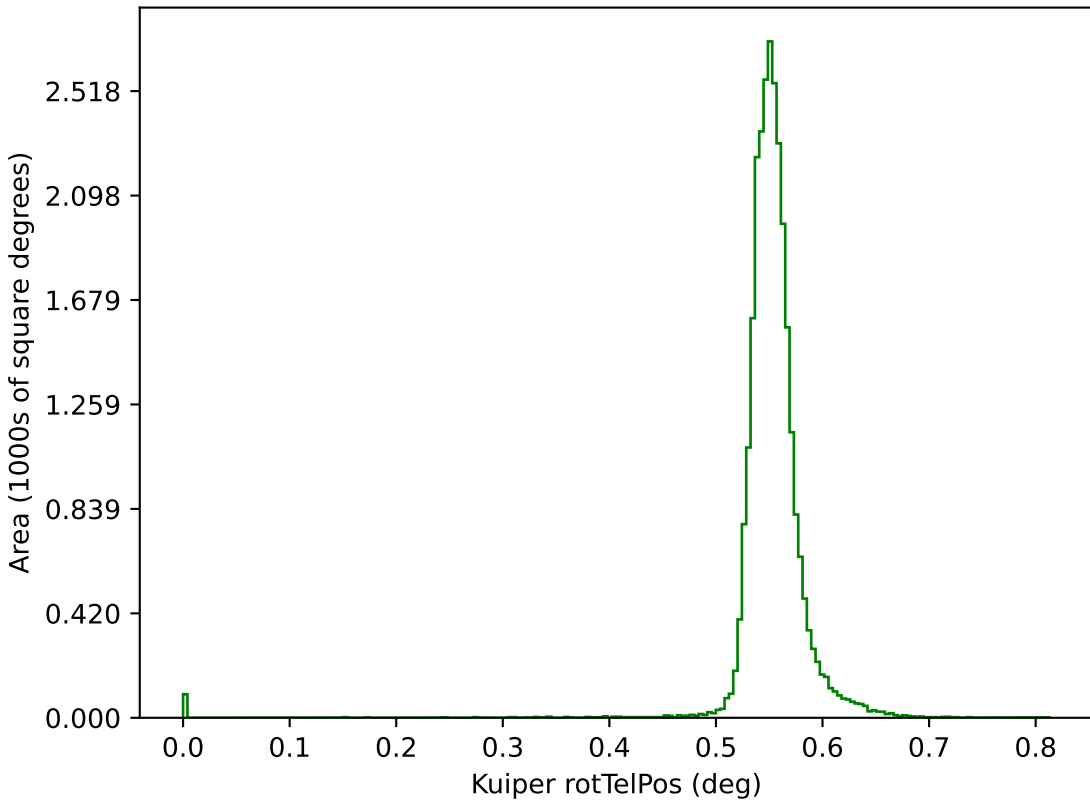
too_elab_r32_d3_giz_v3.4_10yrs g: Kuiper rotTelPos
