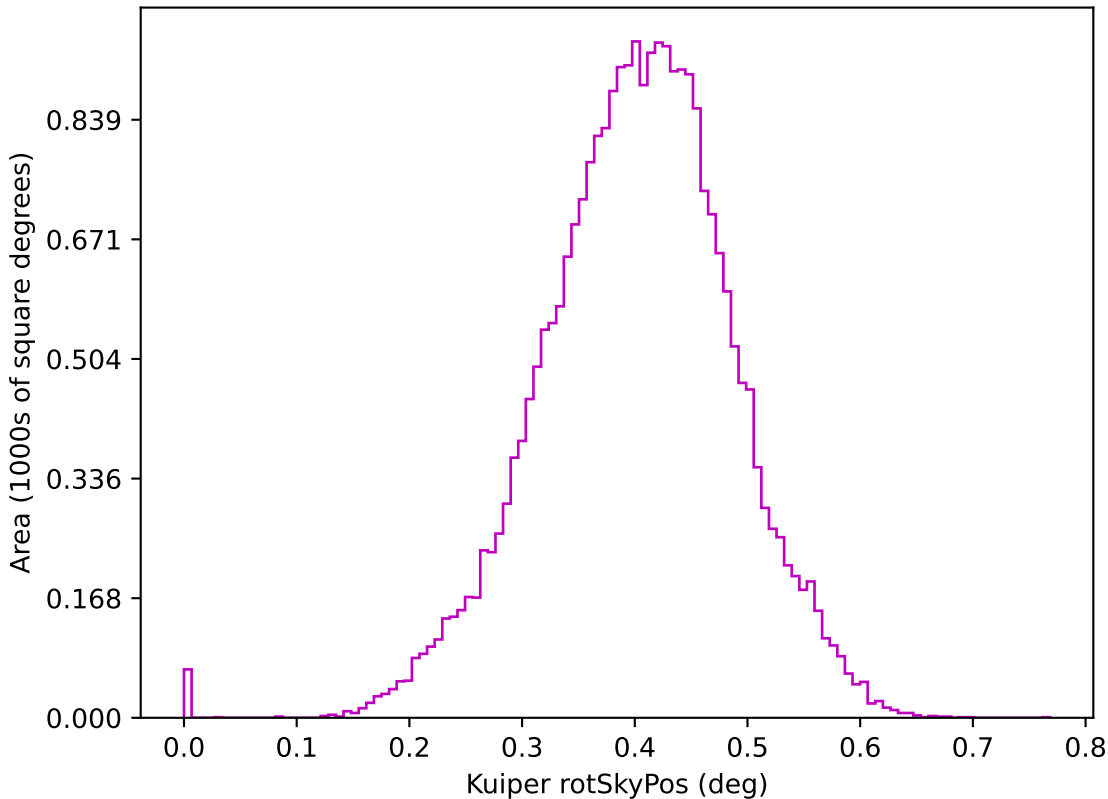
too_elab_r32_d3_giz_v3.4_10yrs z: Kuiper rotSkyPos
