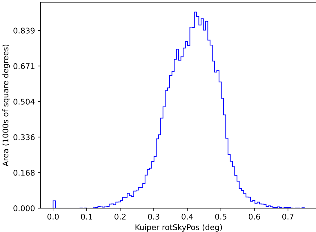
too_elab_r32_d3_giz_v3.4_10yrs y: Kuiper rotSkyPos
