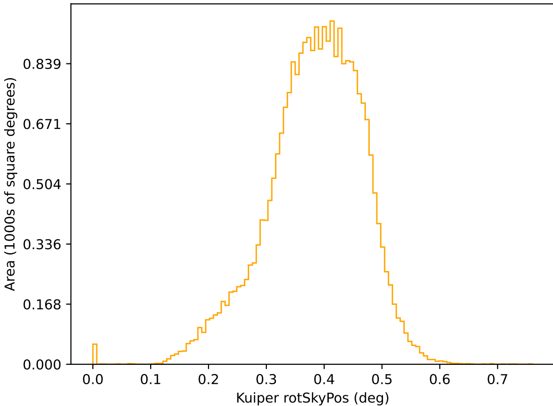
too_elab_r32_d3_giz_v3.4_10yrs r: Kuiper rotSkyPos
