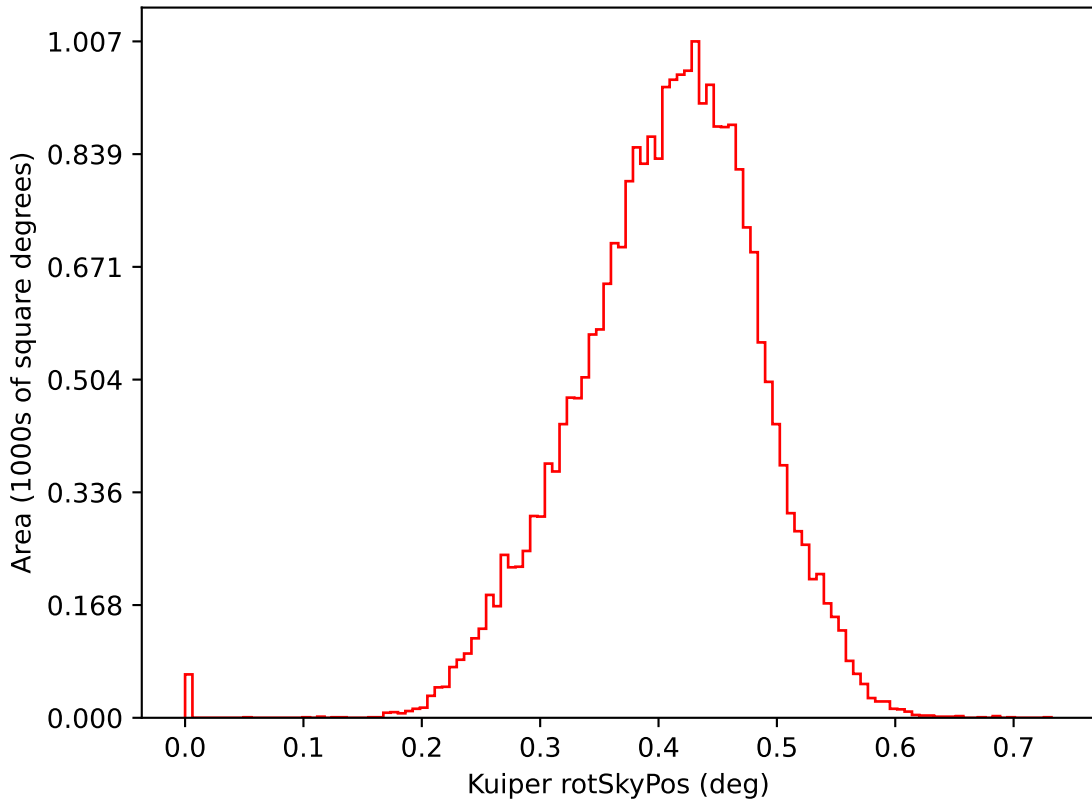
too_elab_r32_d3_giz_v3.4_10yrs i: Kuiper rotSkyPos
