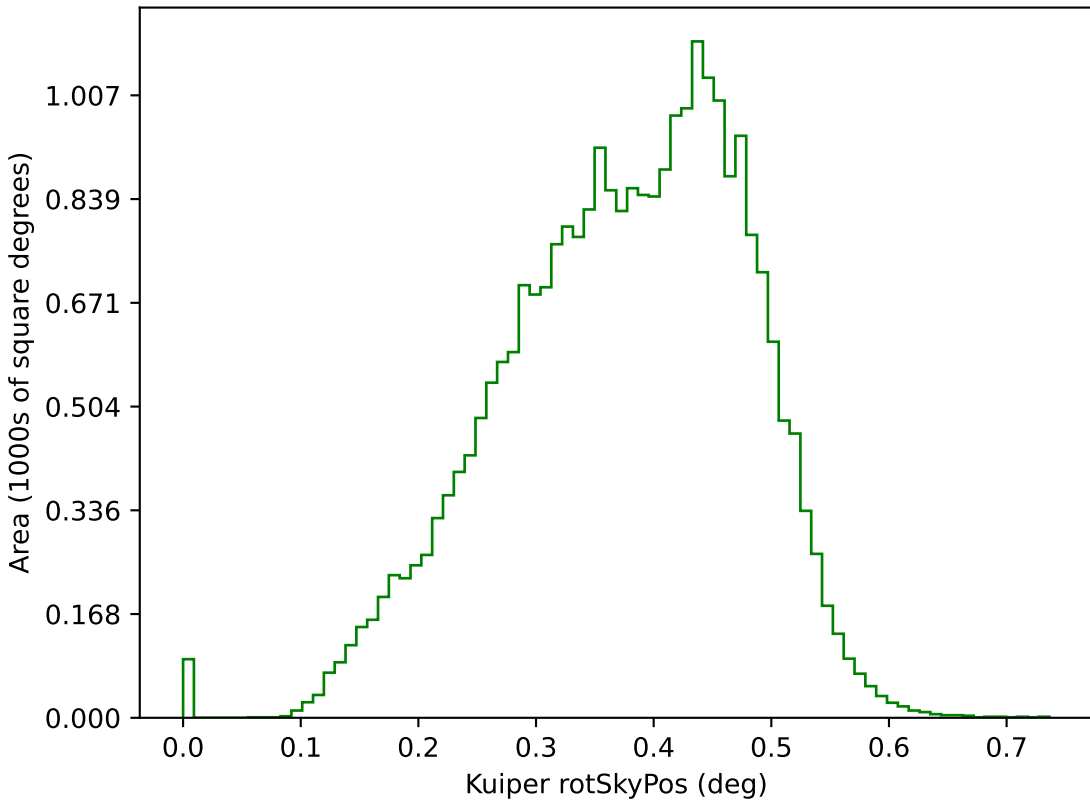
too_elab_r32_d3_giz_v3.4_10yrs g: Kuiper rotSkyPos
