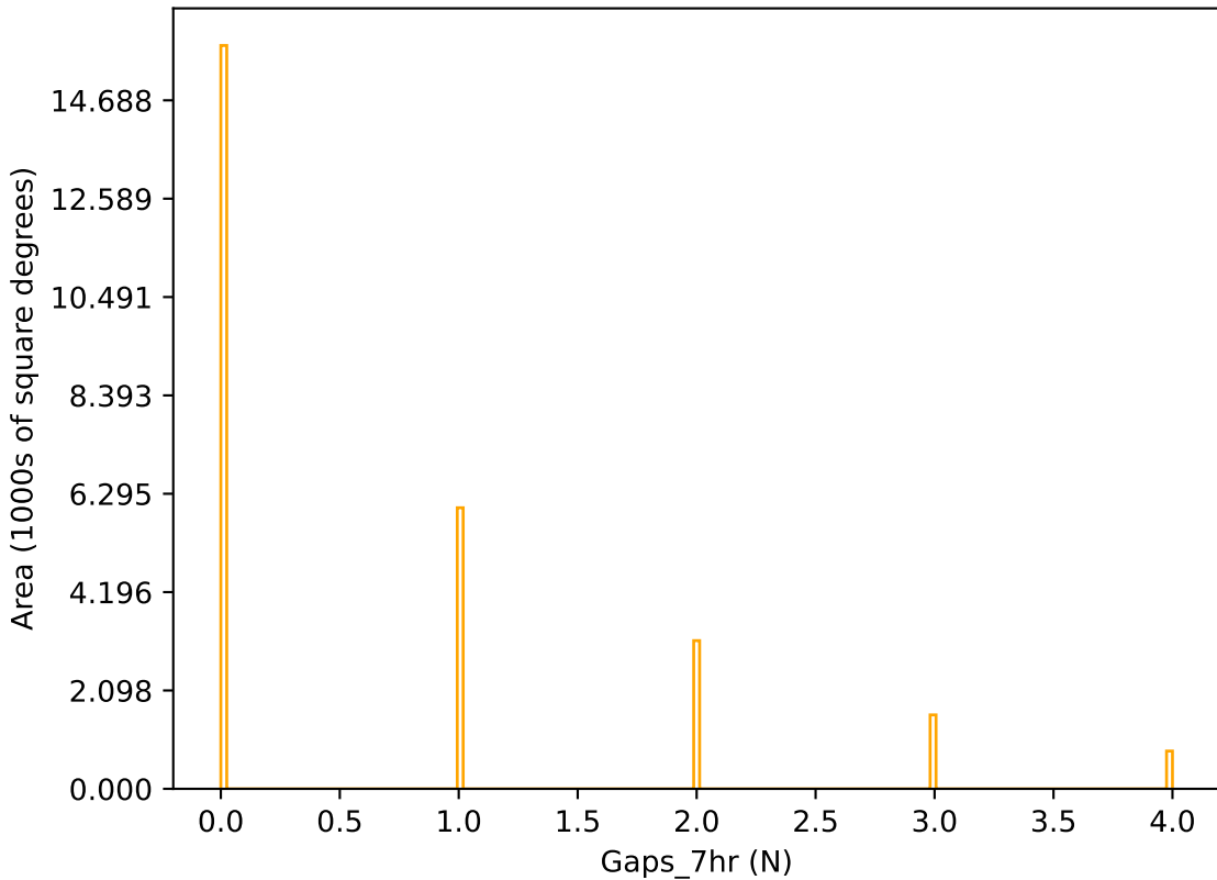
too_elab_r32_d3_giz_v3.4_10yrs r band: Gaps_7hr
