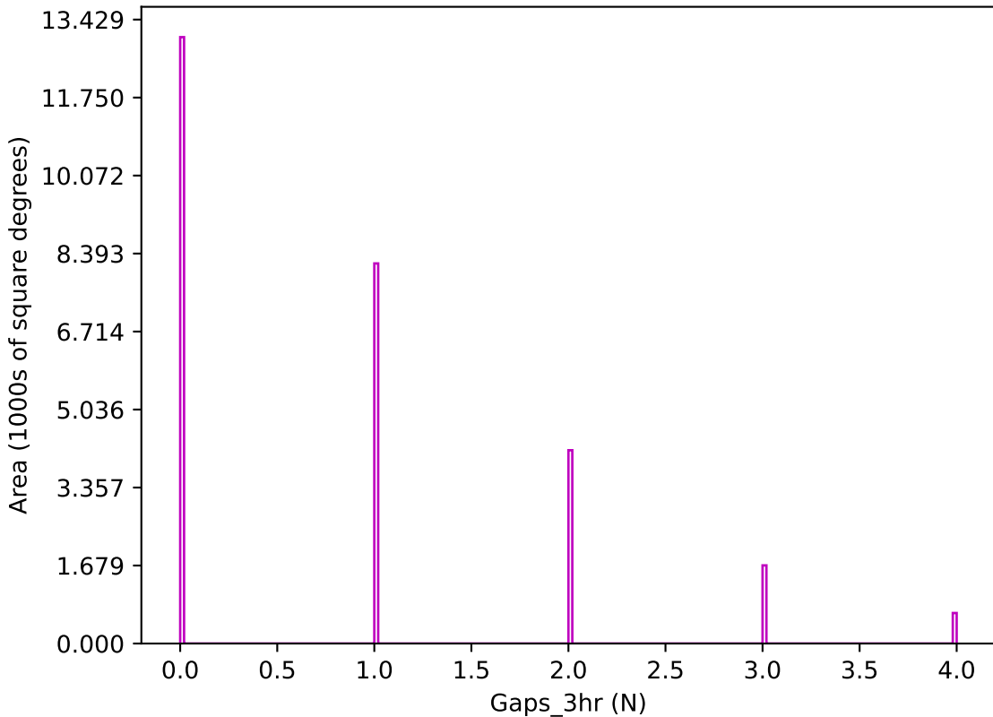
too_elab_r32_d3_giz_v3.4_10yrs z band: Gaps_3hr
