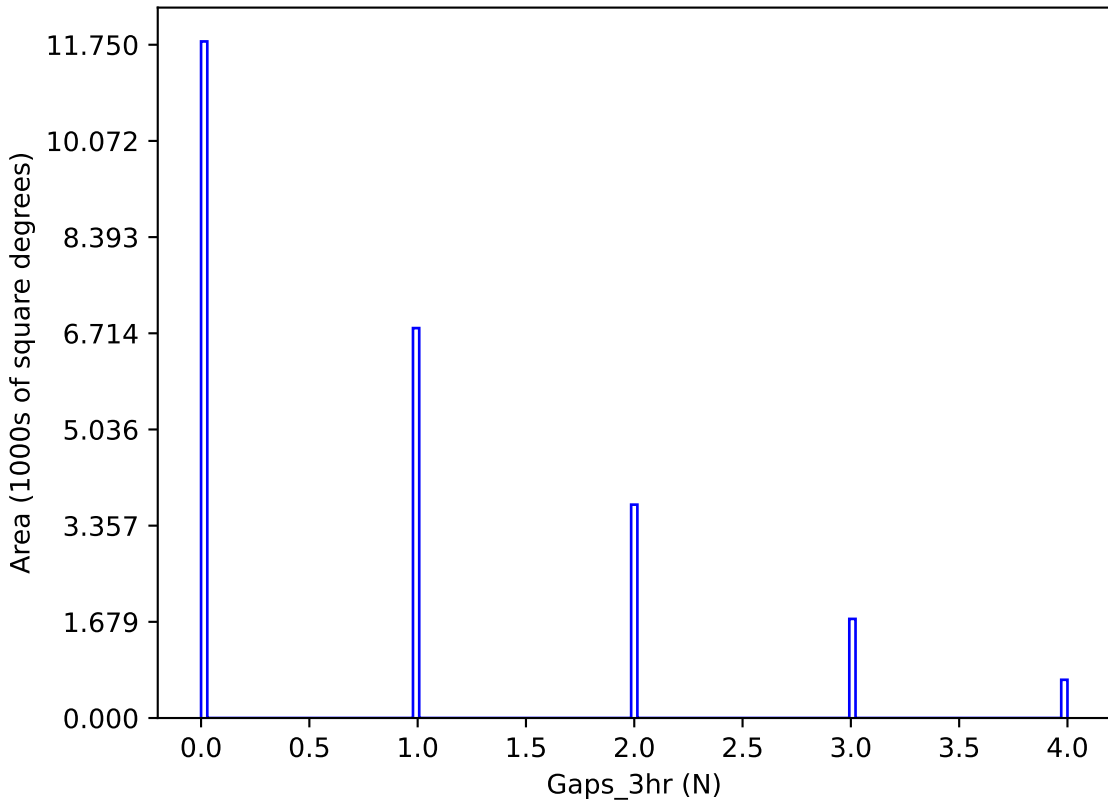
too_elab_r32_d3_giz_v3.4_10yrs y band: Gaps_3hr
