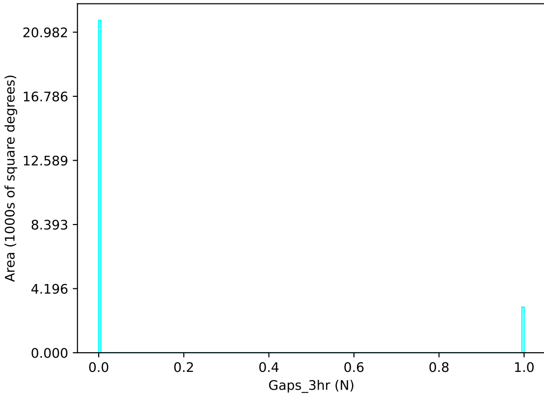
too_elab_r32_d3_giz_v3.4_10yrs u band: Gaps_3hr
