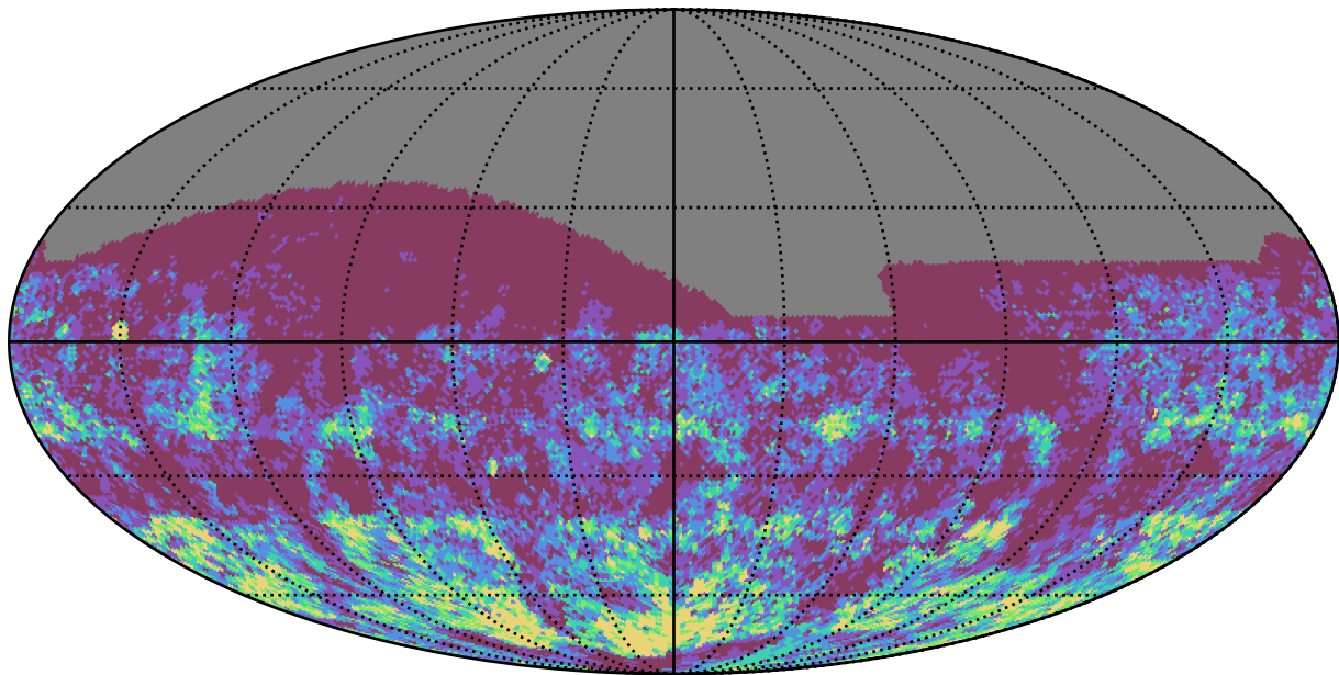
too_elab_r32_d3_giz_v3.4_10yrs r band: Gaps_3hr
