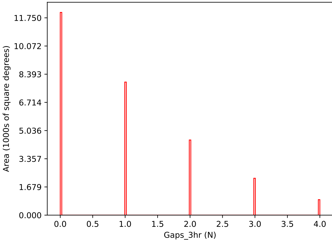
too_elab_r32_d3_giz_v3.4_10yrs i band: Gaps_3hr
