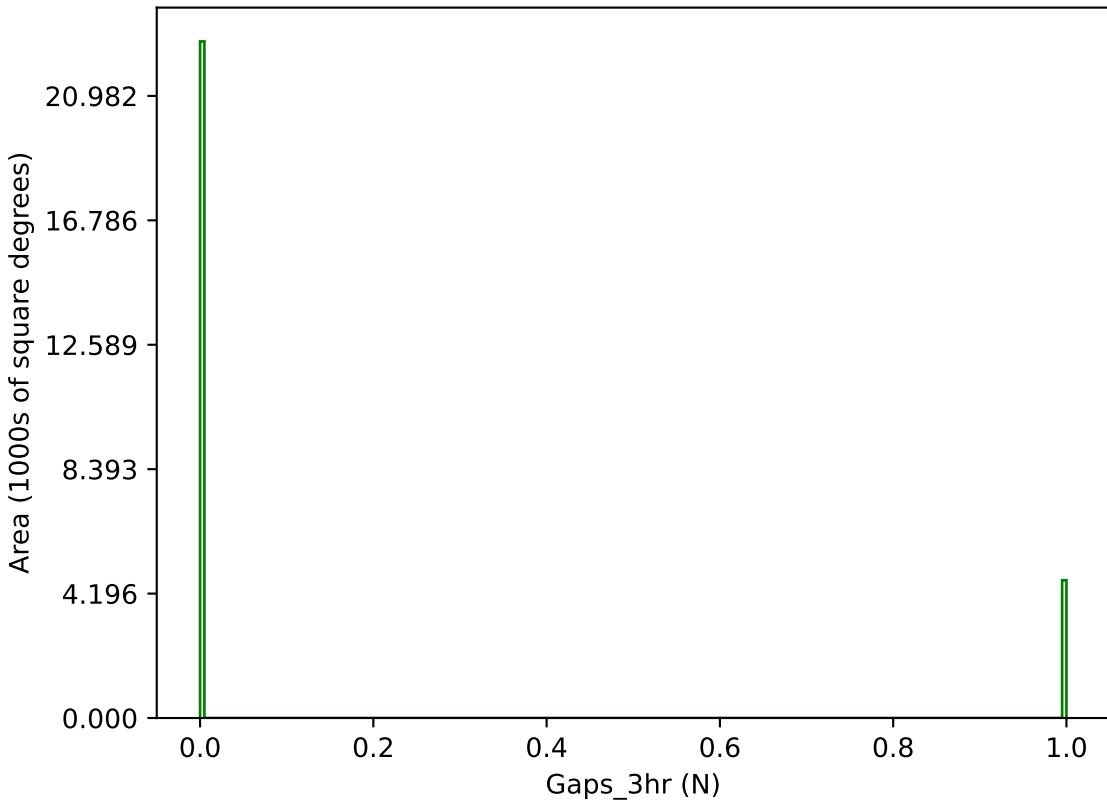
too_elab_r32_d3_giz_v3.4_10yrs g band: Gaps_3hr
