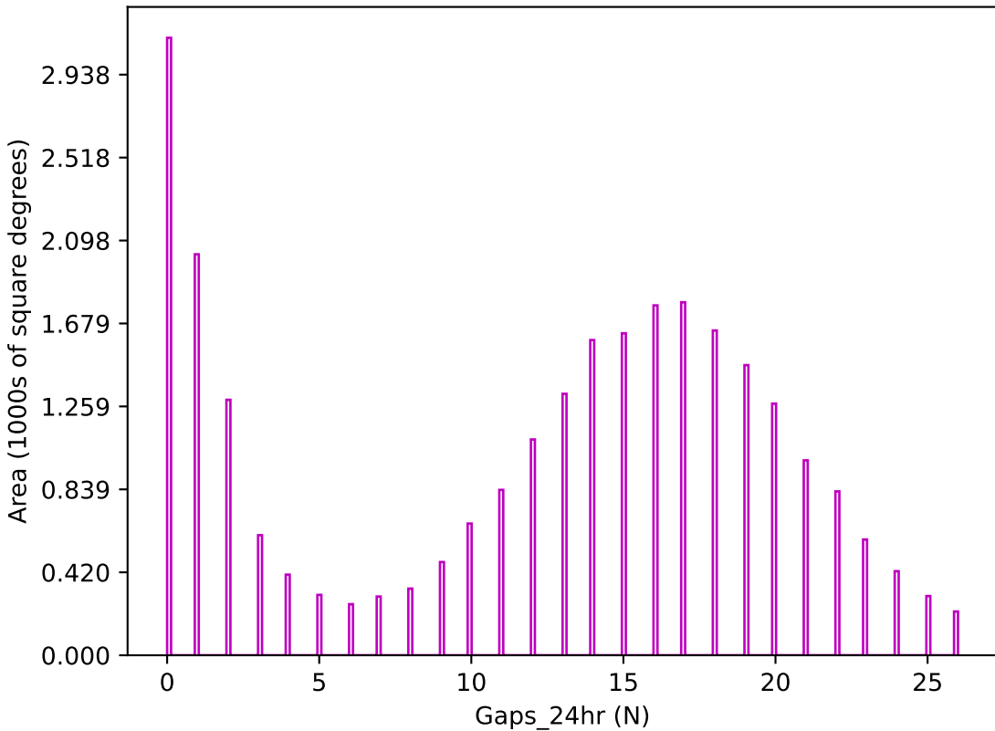
too_elab_r32_d3_giz_v3.4_10yrs z band: Gaps_24hr
