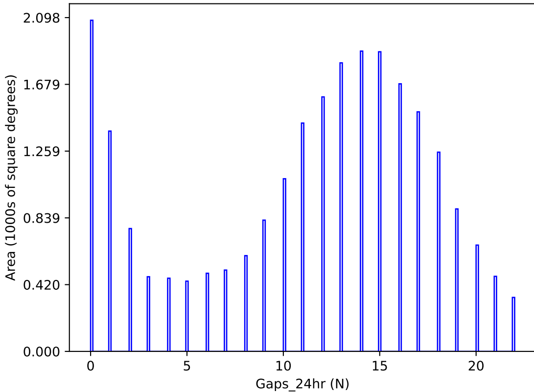
too_elab_r32_d3_giz_v3.4_10yrs y band: Gaps_24hr
