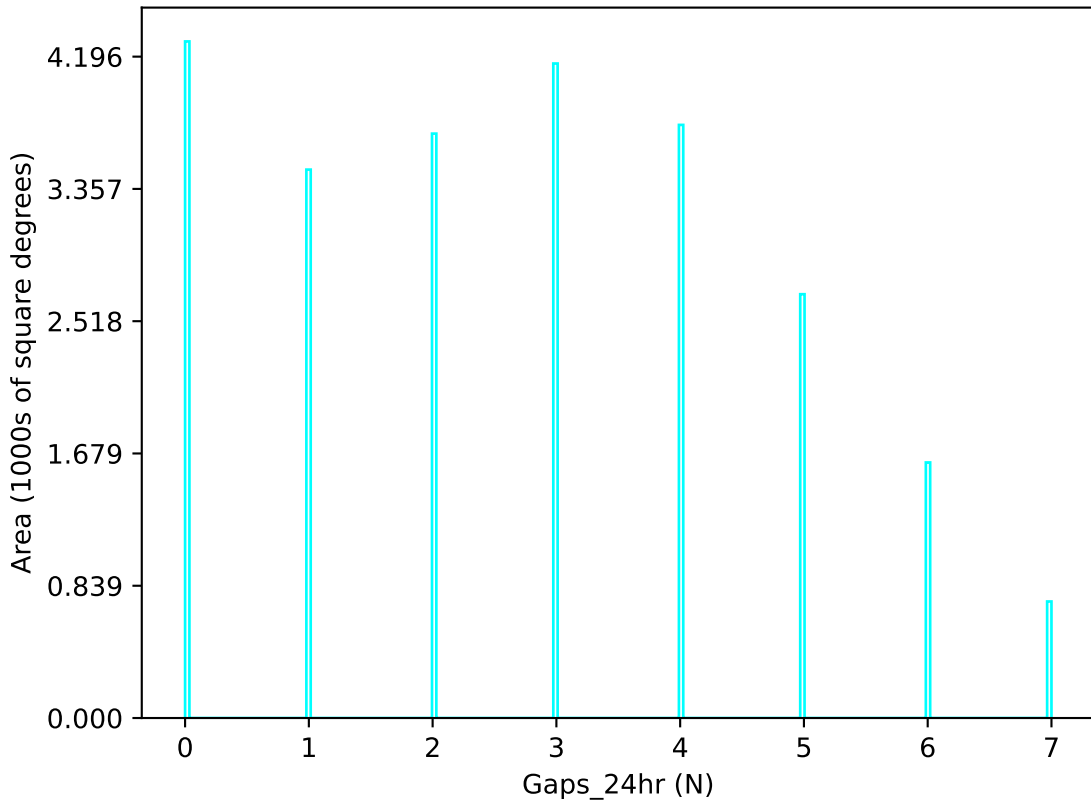
too_elab_r32_d3_giz_v3.4_10yrs u band: Gaps_24hr
