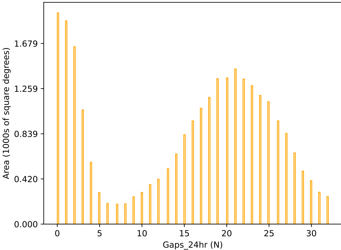
too_elab_r32_d3_giz_v3.4_10yrs r band: Gaps_24hr
