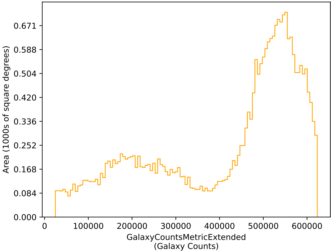
too_elab_r32_d3_giz_v3.4_10yrs r: GalaxyCountsMetricExtended
