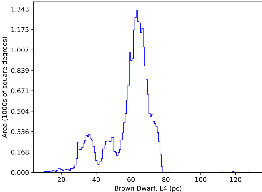
too_elab_r32_d3_giz_v3.4_10yrs : Brown Dwarf, L4
