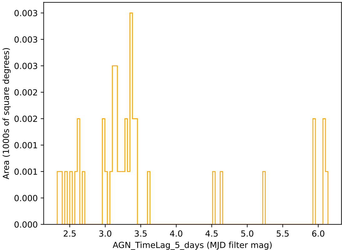
too_elab_r32_d3_giz_v3.4_10yrs r band: AGN_TimeLag_5_days
