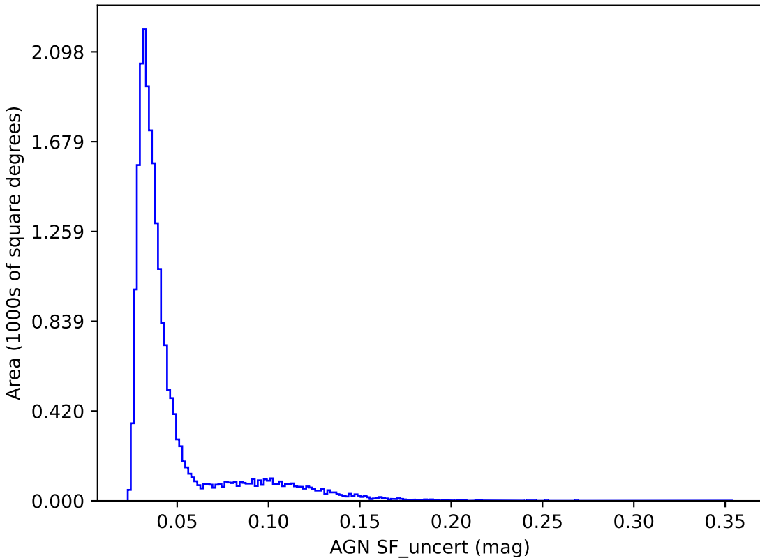
too_elab_r32_d3_giz_v3.4_10yrs y band: AGN SF_uncert
