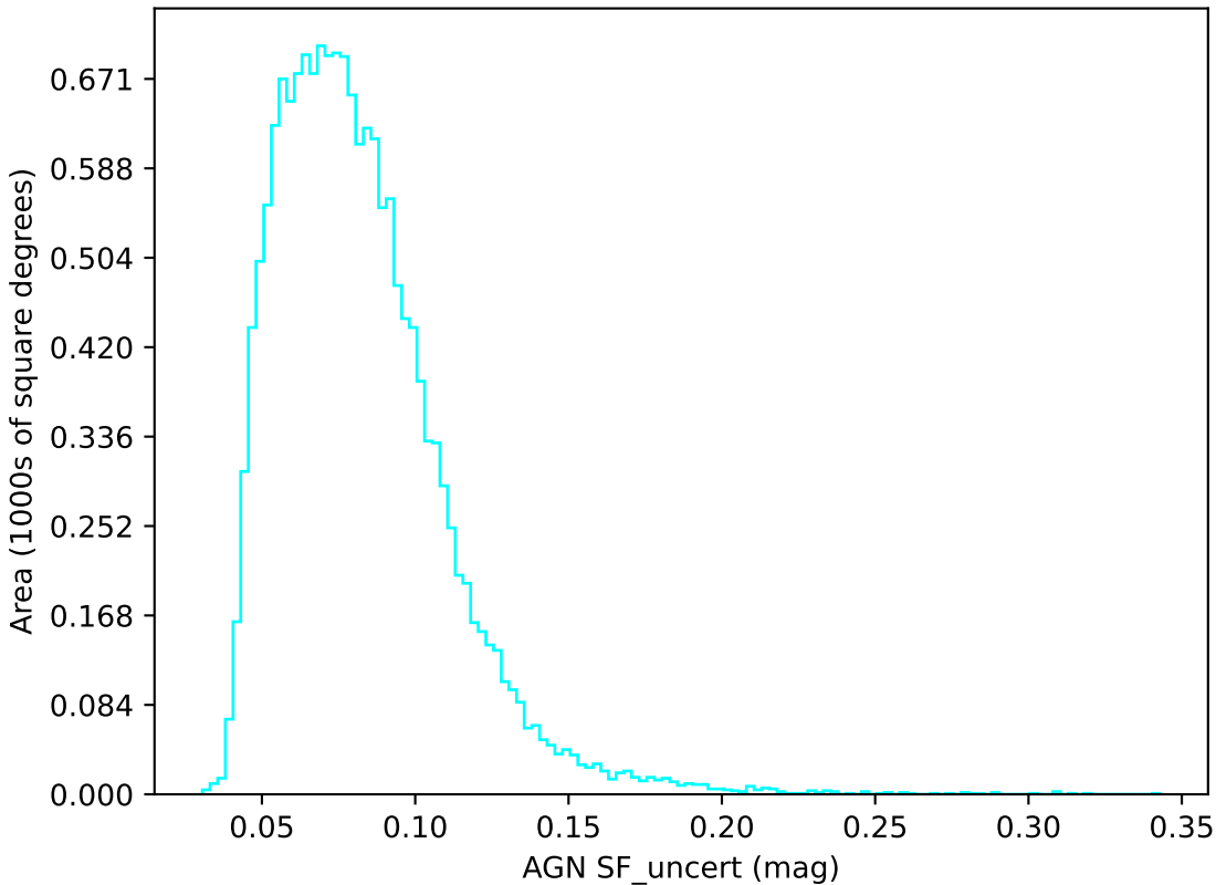
too_elab_r32_d3_giz_v3.4_10yrs u band: AGN SF_uncert
