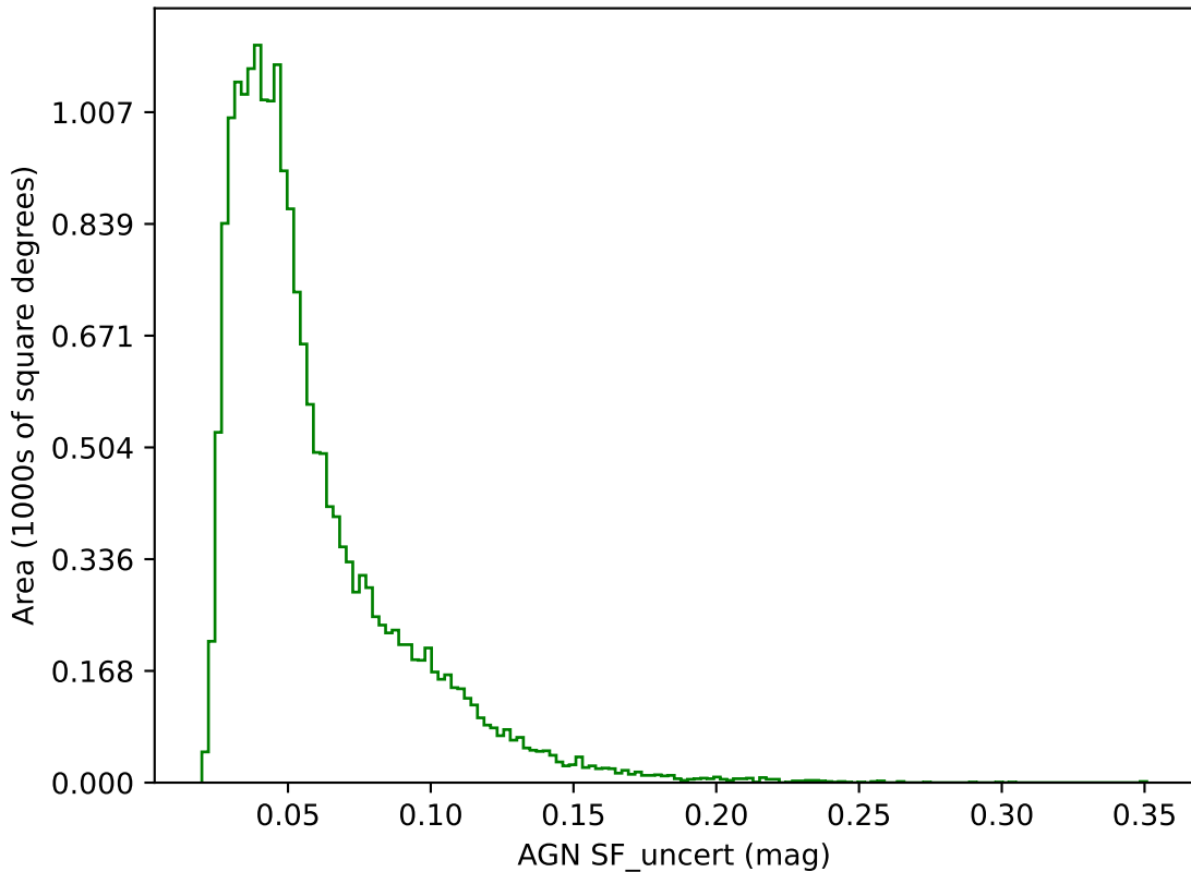
too_elab_r32_d3_giz_v3.4_10yrs g band: AGN SF_uncert
