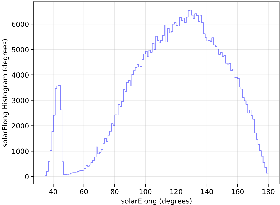
too_elab_r32_d3_giz_v3.4_10yrs WFD z band: solarElong Histogram
