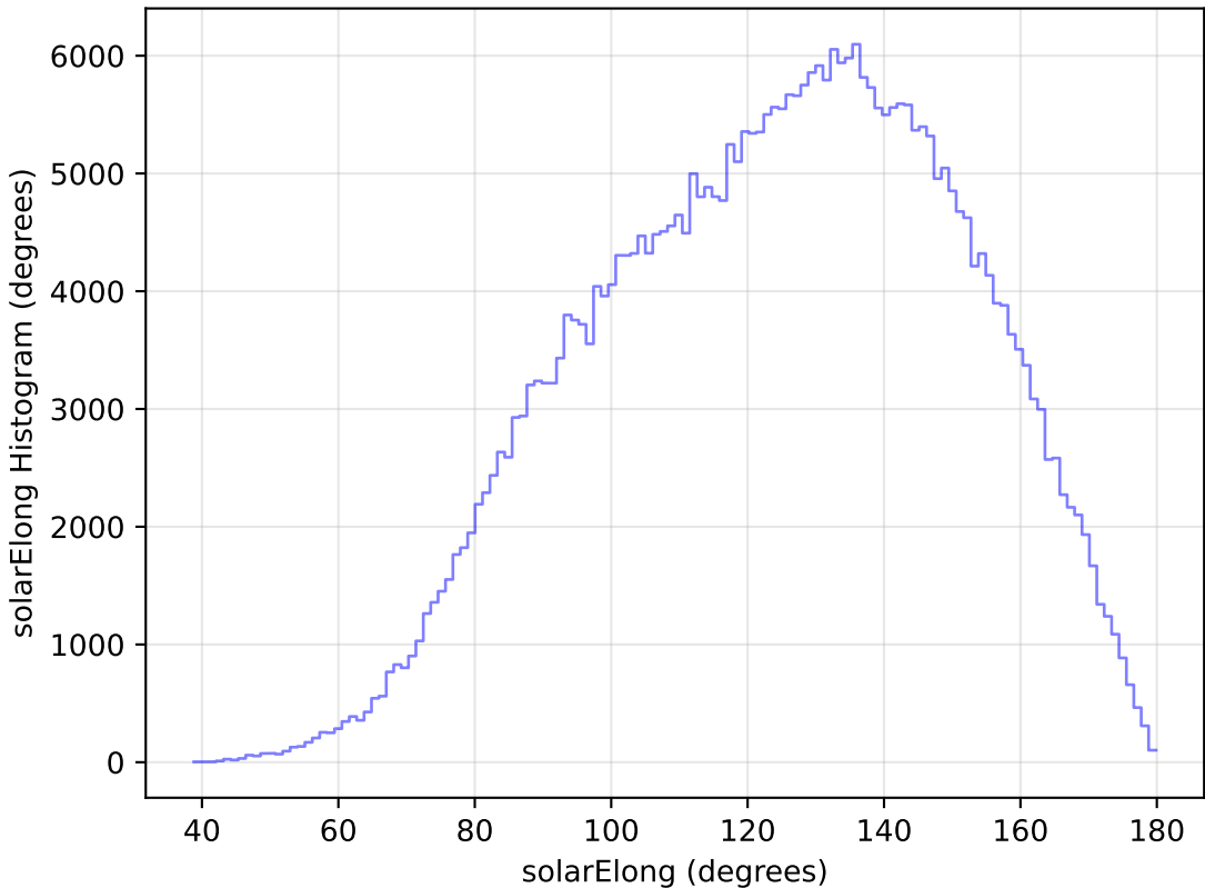
too_elab_r32_d3_giz_v3.4_10yrs WFD y band: solarElong Histogram
