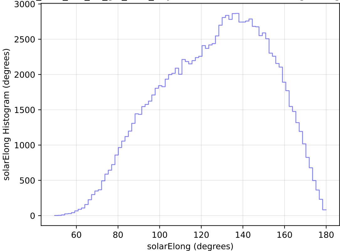
too_elab_r32_d3_giz_v3.4_10yrs WFD u band: solarElong Histogram
