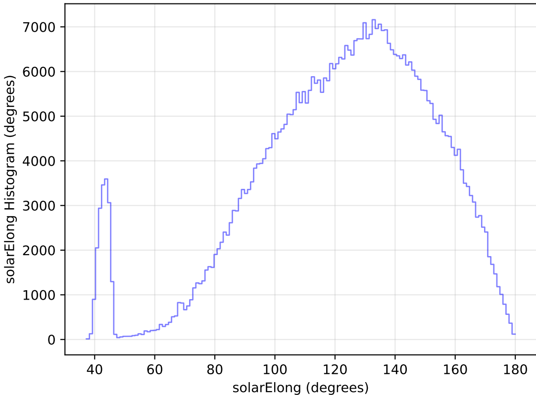
too_elab_r32_d3_giz_v3.4_10yrs WFD r band: solarElong Histogram
