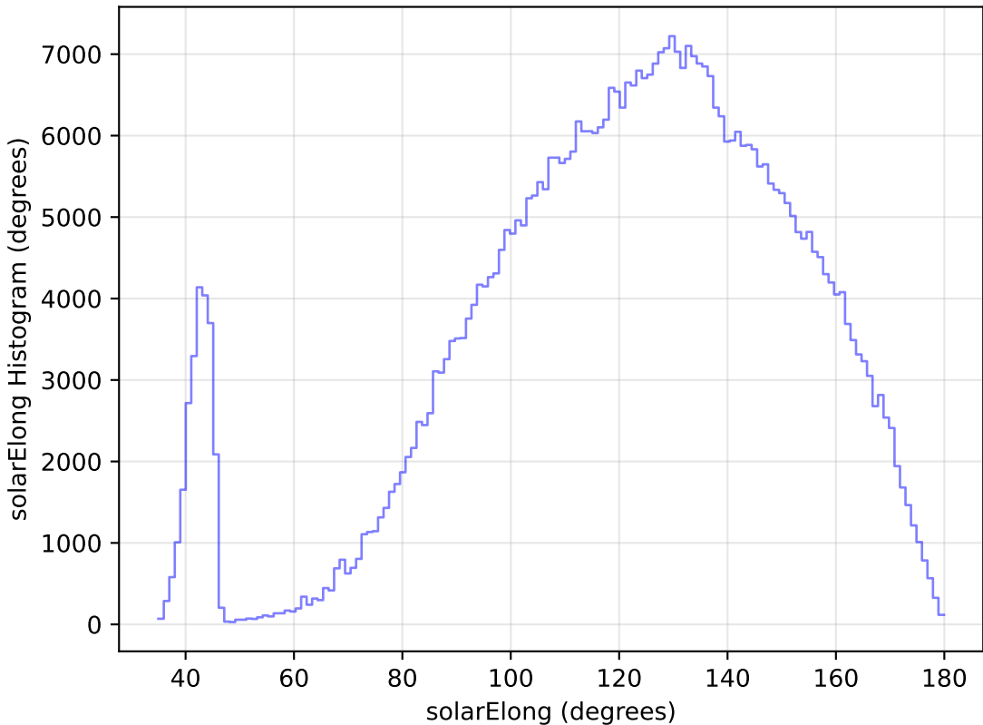
too_elab_r32_d3_giz_v3.4_10yrs WFD i band: solarElong Histogram
