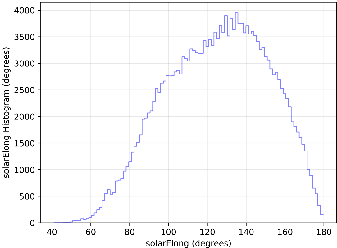
too_elab_r32_d3_giz_v3.4_10yrs WFD g band: solarElong Histogram
