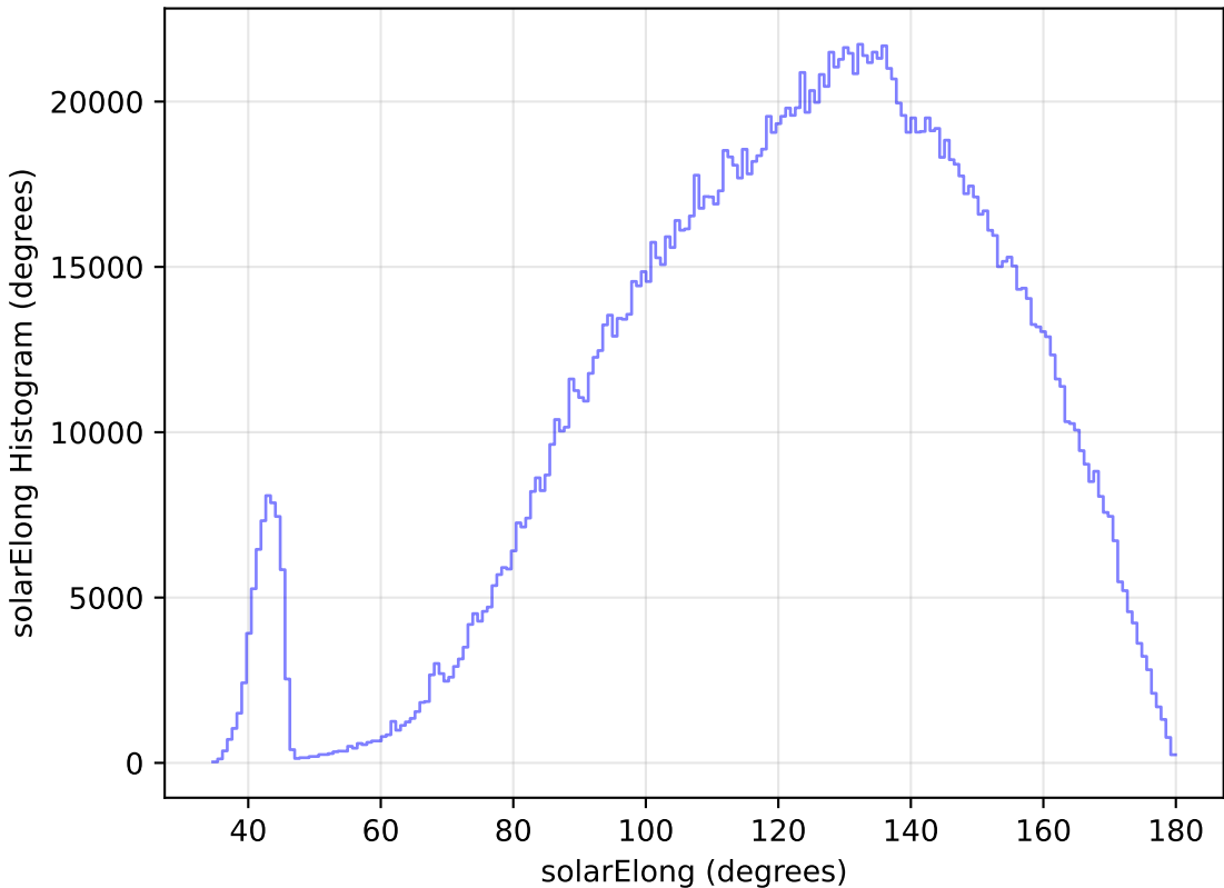
too_elab_r32_d3_giz_v3.4_10yrs WFD all bands: solarElong Histogram
